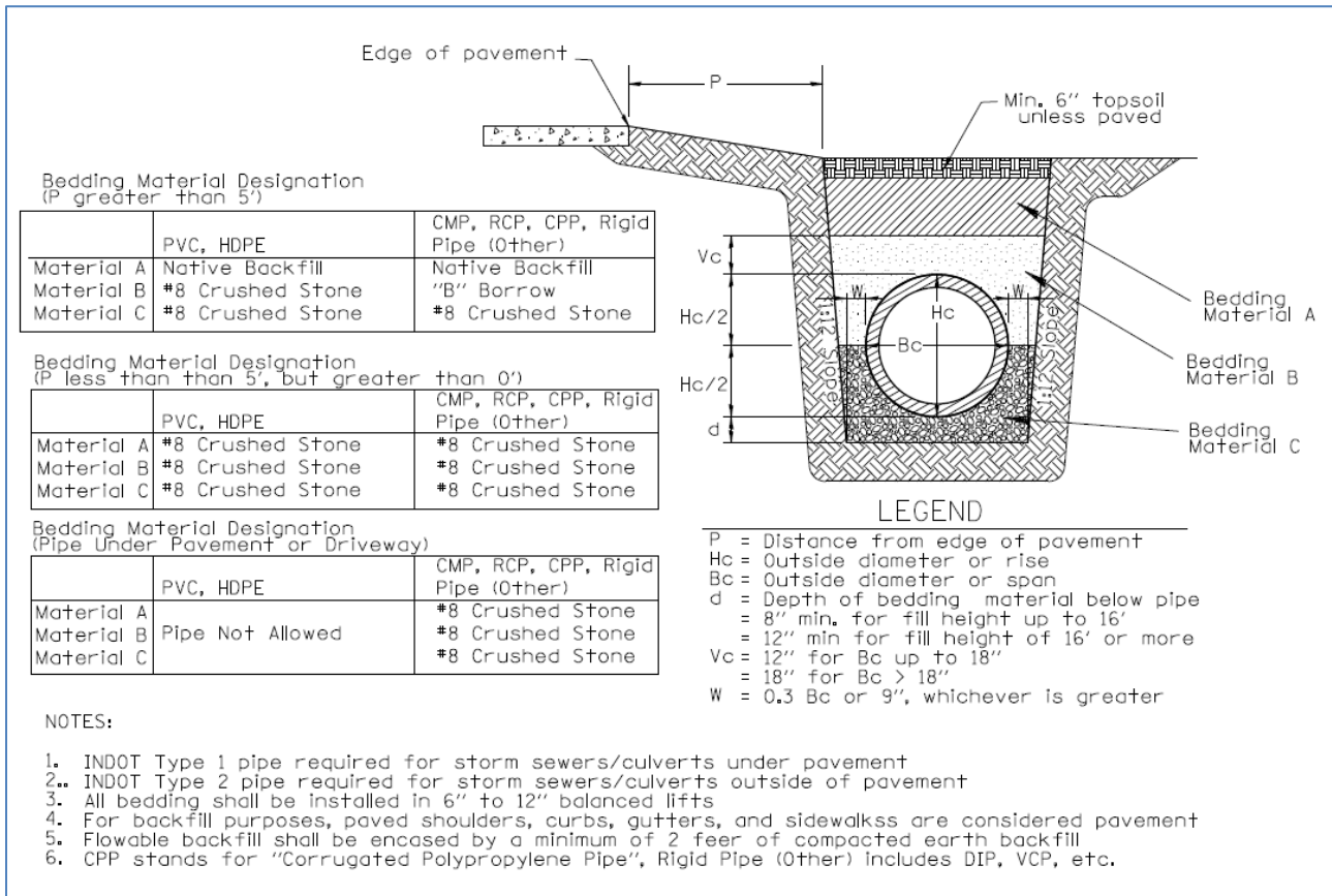
FIGURE 4-1 Example Bedding and Backfill Standards for Storm Sewers*
