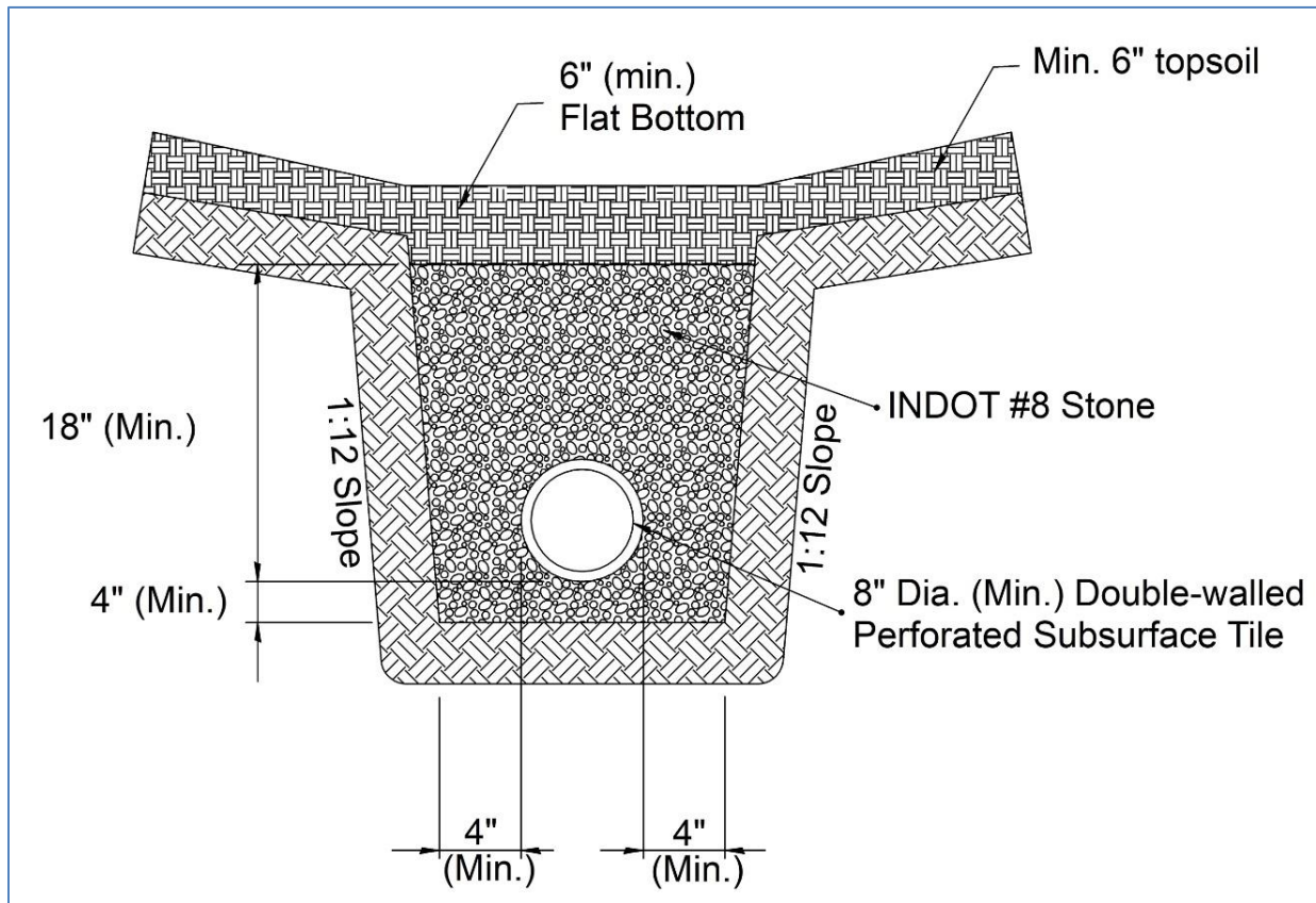
FIGURE 4-2 Example Bedding and Backfill Standards for Sub-drains under Swales
